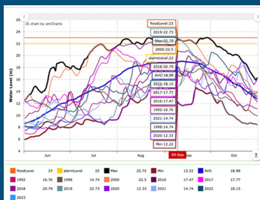
Historical data of Peak Flows of the Mekong River in Kratié (Mekong River Commission, 2024)
